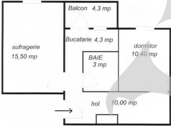
APARTAMENT 2 CAMERE 47.7 mp
